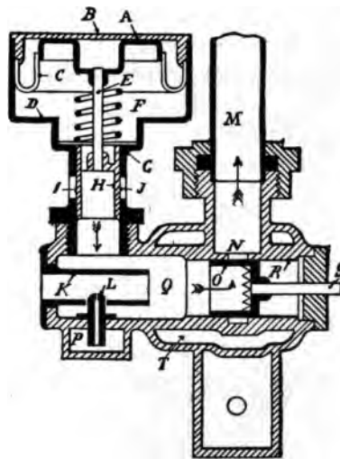
FIG. 161.—Section of the Krebs Mixer used with the later Panhard-Levassor Engines. The float chamber and other parts are identical with the Centaure carburetter. Gasoline comes from the float chamber through channel, P , and spraying nozzle, L , air being admitted at K . Q is the mixing chamber from which the air and gasoline gas passes into the feed tube, M , through the port, H , whose opening is controlled by the position of the serrated perforations in piston, O , moving through bore, R , as controlled by the governor through piston rod, S . When more air than the fixed quantity admitted at K is required by the conditions of motor operation, the suction of the motor piston depresses the small piston, A , held in cylinder, F , by the spring, E , and sliding in the elastic diaphragm, C . Air is admitted above it through a small port at B . The depression of piston, A , and causes the slide, H , to move downward in tube, G , thus opening to a greater or less degree the ports, J and J , admitting the required amount of air for any given condition.
